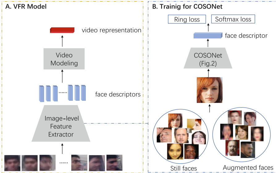
Fig. 1. Left is the general VFR model composed of two parts: image-level feature extractor and video modeling module. Right is the pipeline of training COSONet. Each training image in a batch is either picked from still faces or video-like augmented ones. The COSONet is trained with two losses: softmax loss and ring loss.
