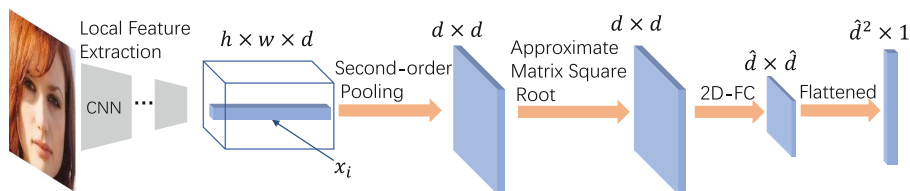
Fig. 2. The network structure of COSONet.
