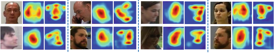
Fig. 4. In each group, the first is the inputed face image, the second and the third are the corresponding averaged feature maps along the channel dimension of the plain first-order network and our COSONet. The two feature maps are respectively from the output of the fourth block convolution layer of Model A and Model B (in Sect. 4.4).
